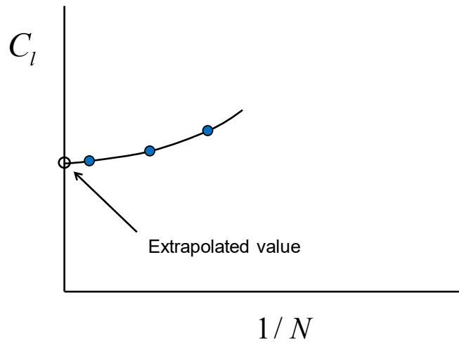
Fig. 1. Illustration of the extrapolation process. The three blue dots are the data points, corresponding to the three different values of N . The white dot is the extrapolated value.
