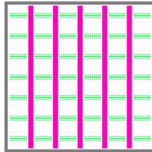
TE 10 mode of square waveguide
